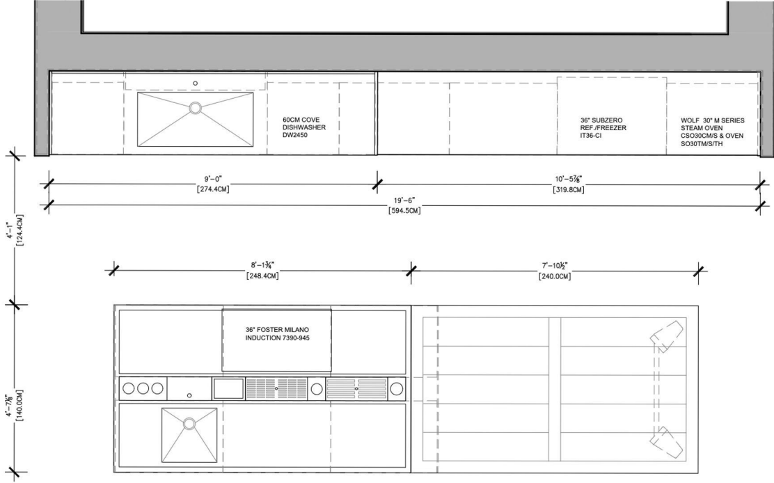
CONVIVUM KITCHEN DISPLAY PLAN
