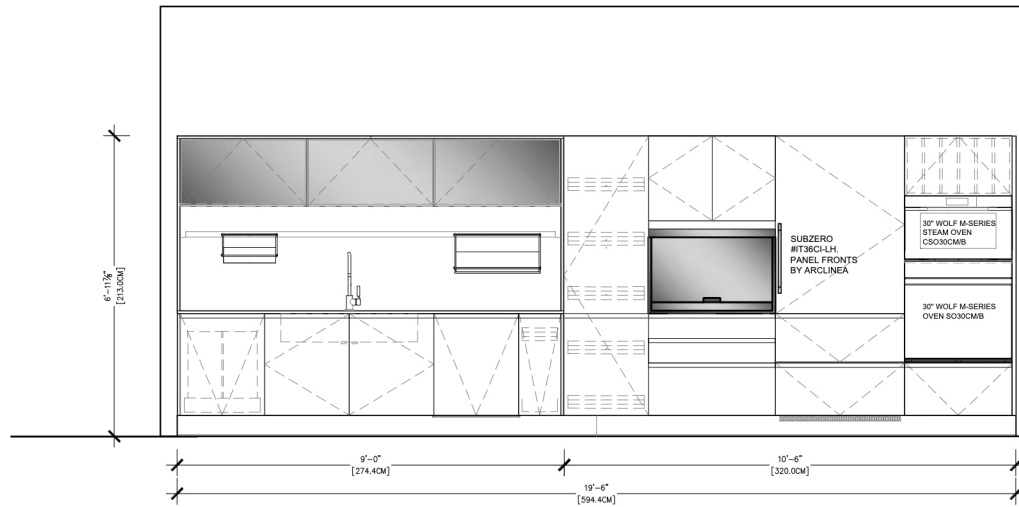
CONVIVIUUM SINK TALL WALL ELEVATION
