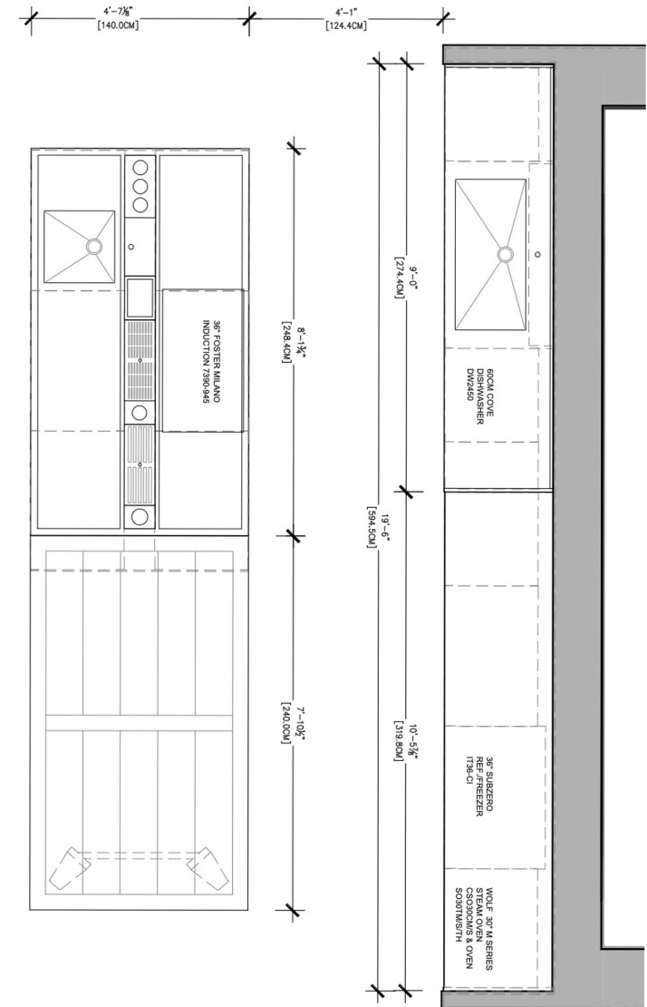
CONVIVIUUM KITCHEN DISPLAY PLAN
