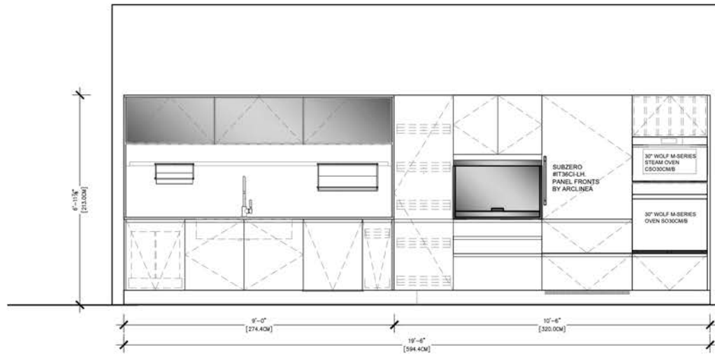
CONVIVIUM SINK TALL WALL ELEVATION
